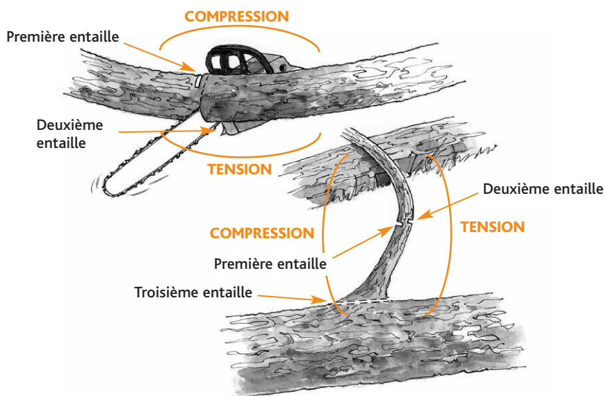
Illustration n° 40 Tension-compression
