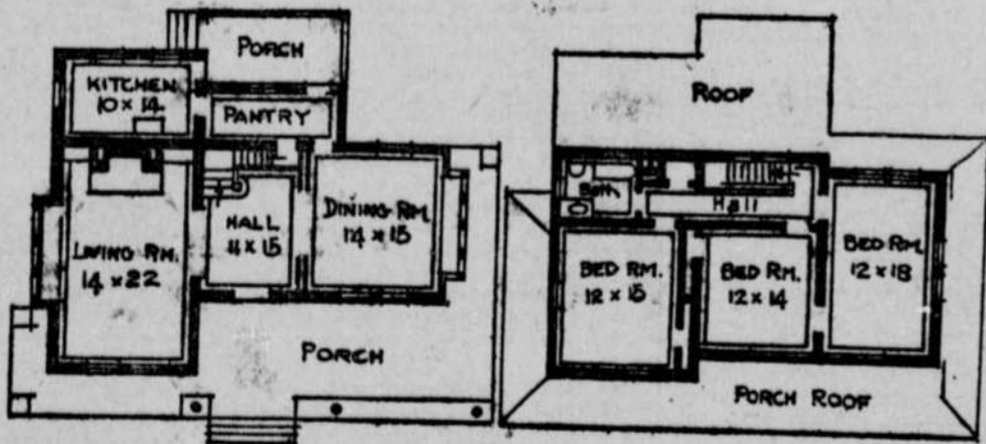
- FIRST FLOOR PLAN - - SECOND FLOOR PLAN -
