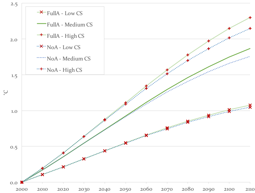
Figure 7: Temperature increase for low, medium, and high CS levels in the FullA and NoA scenarios.
