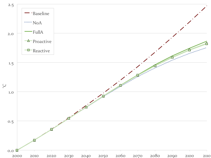
Figure 1: Temperature increase (from 2000).
