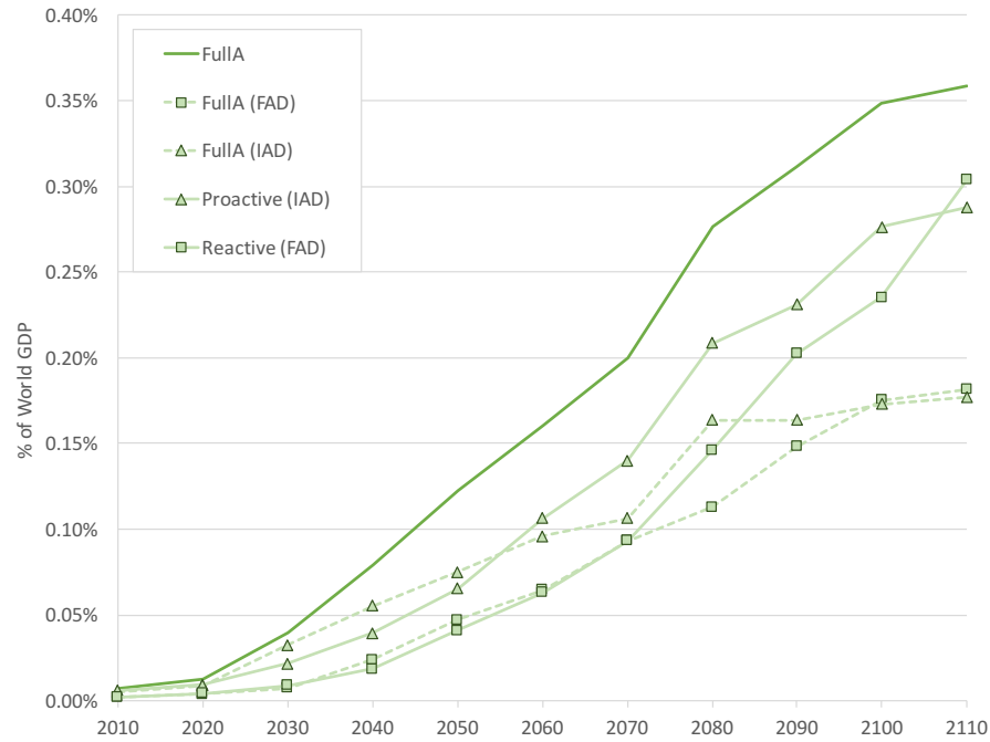
Figure 3: Total adaptation costs (proactive and/or reactive) over time, in % of world GDP. In the FullA scenario, the cost decomposition between proactive and reactive adaptation is given respectively by the dashed lines “FullA (IAD)” and “FullA (FAD)”.
