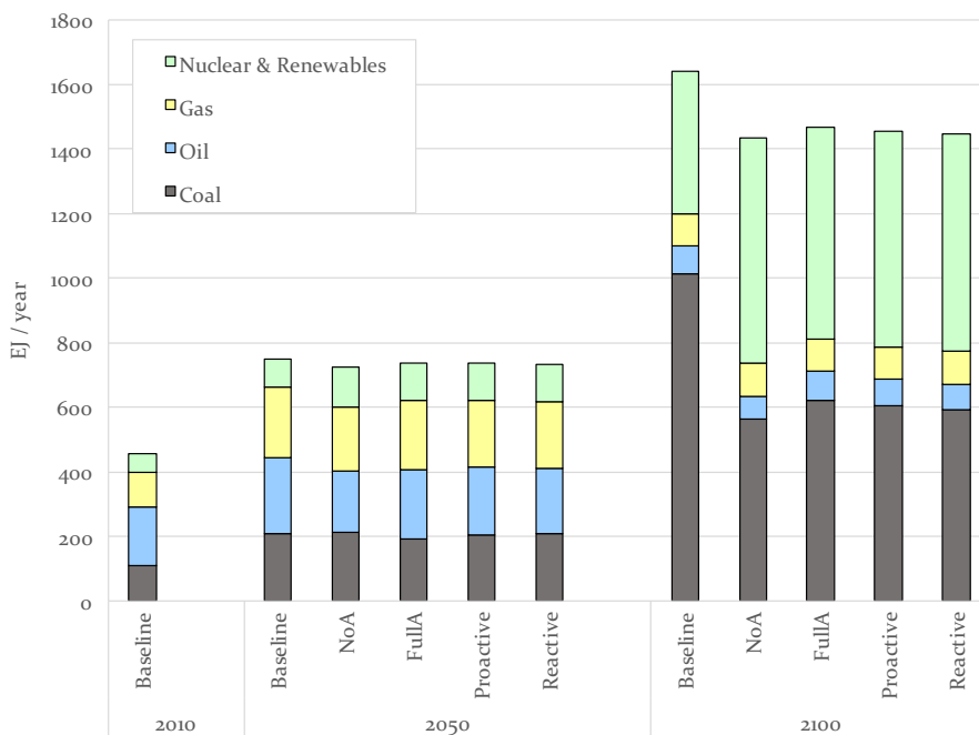
Figure 5: World primary energy use.
