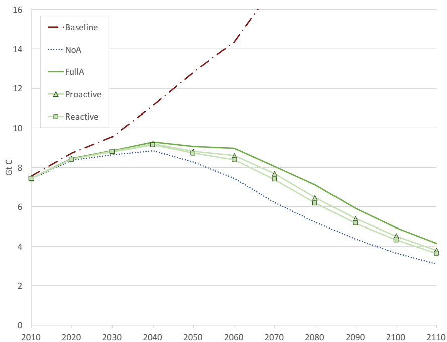
Figure 2: World energy-related CO 2 emission trajectories.
