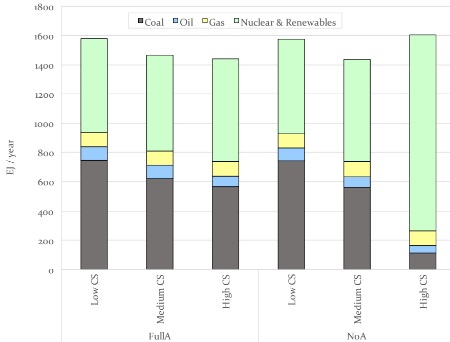
Figure 8: Global primary energy use for low, medium, and high CS levels in the FullA and NoA scenarios.
