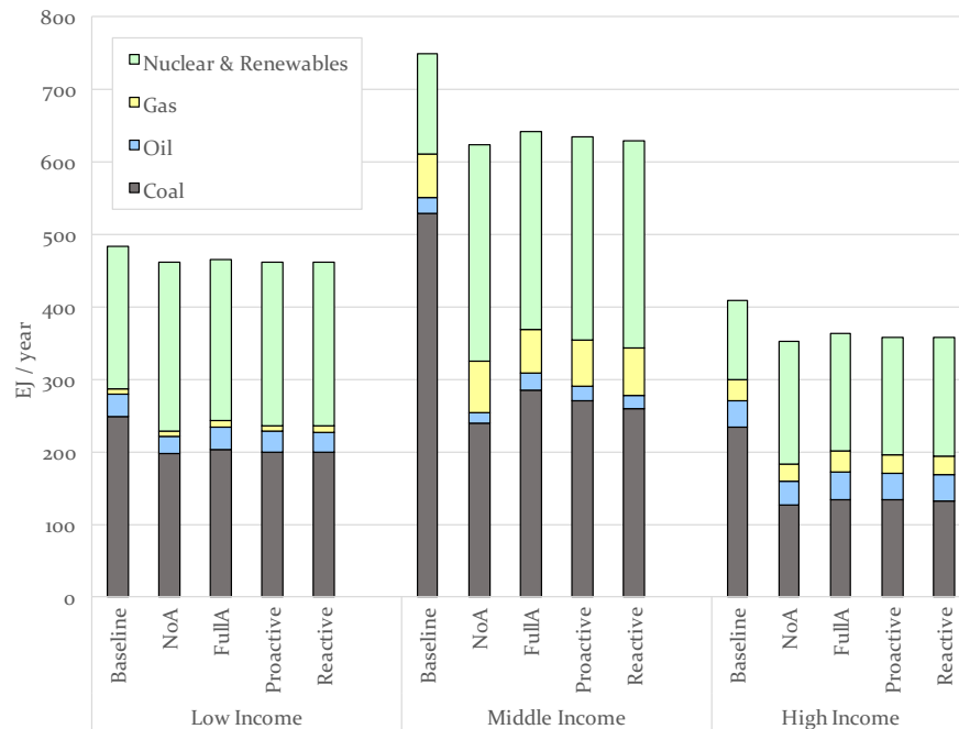
Figure 6: Regional primary energy use.
