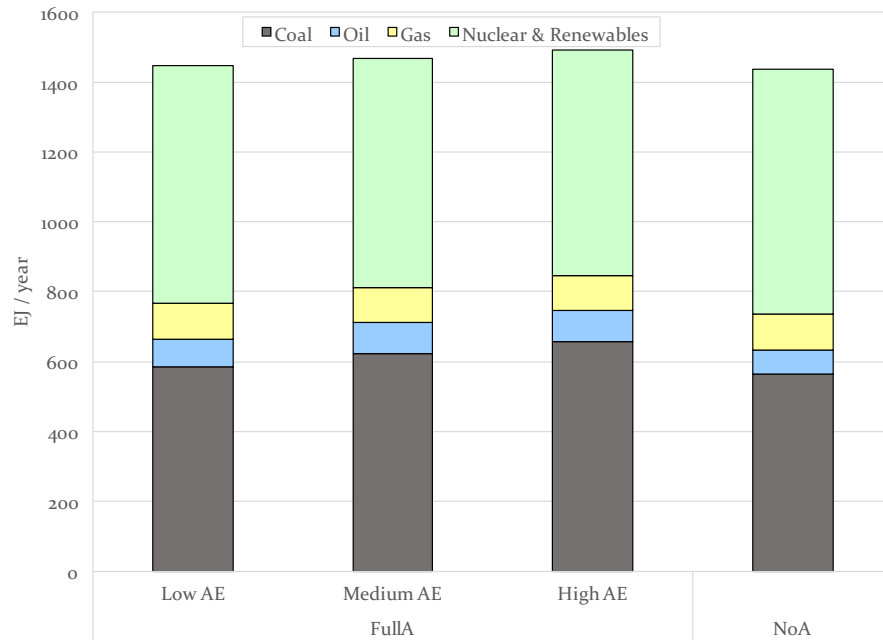
Figure 9: Global primary energy use for low, medium, and high AE levels in the FullA and NoA scenarios.
