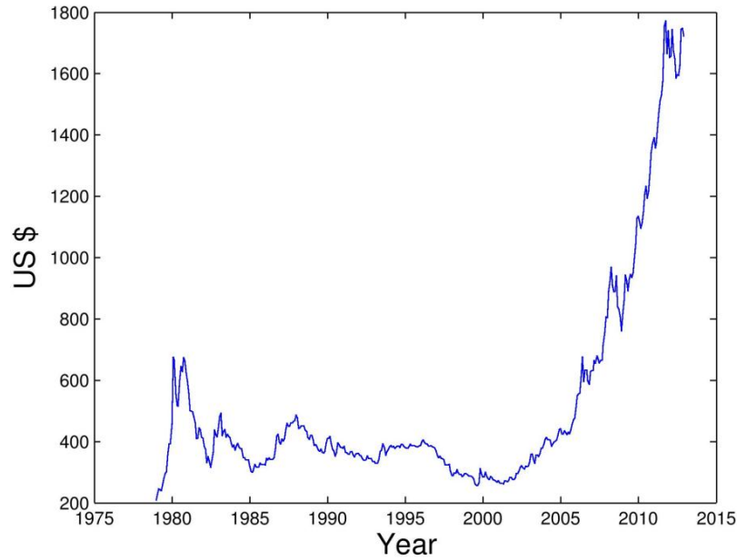
Figure 1: Historical gold price chart
