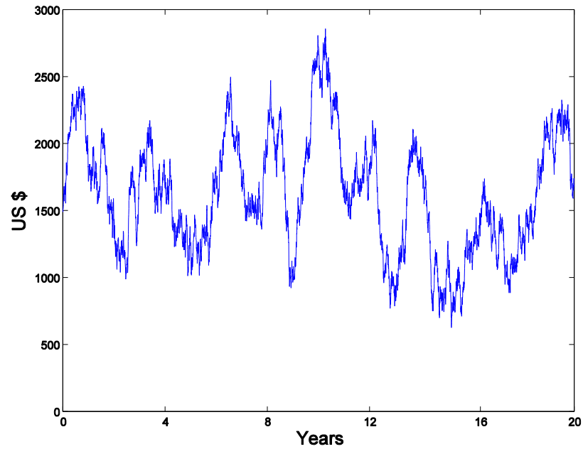
Figure 3: Simulated fictional mine price trajectory
