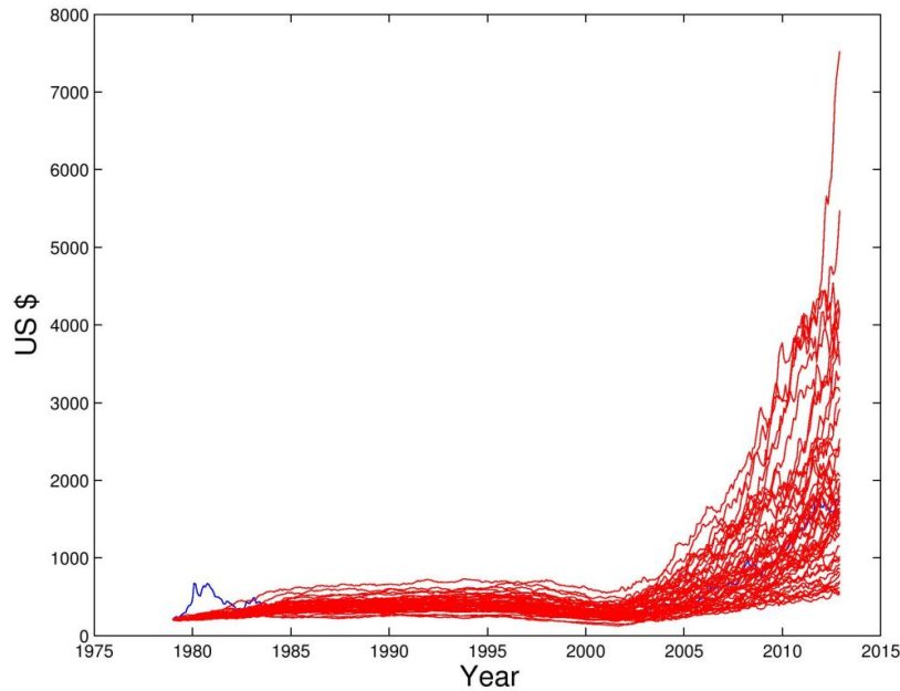
Figure 2: Gold price simulations using the ML estimates
