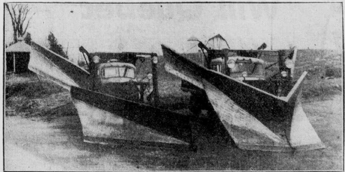
During the winter, C. C. Warner Transport Service specializes in clearing and maintenance of winter roads, and they have been highly complimented for the efficiency of their work. Above are two giant plows pushed by heavy trucks.
